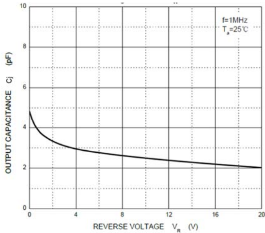
Fig 5: Capacitance Capability
