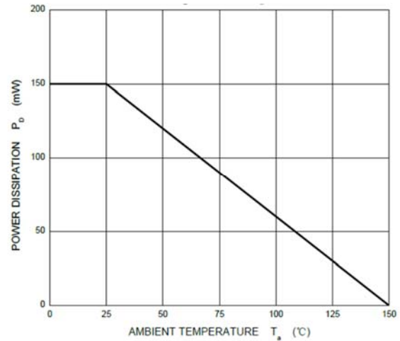
Fig 6: P_D-Ta Curve
