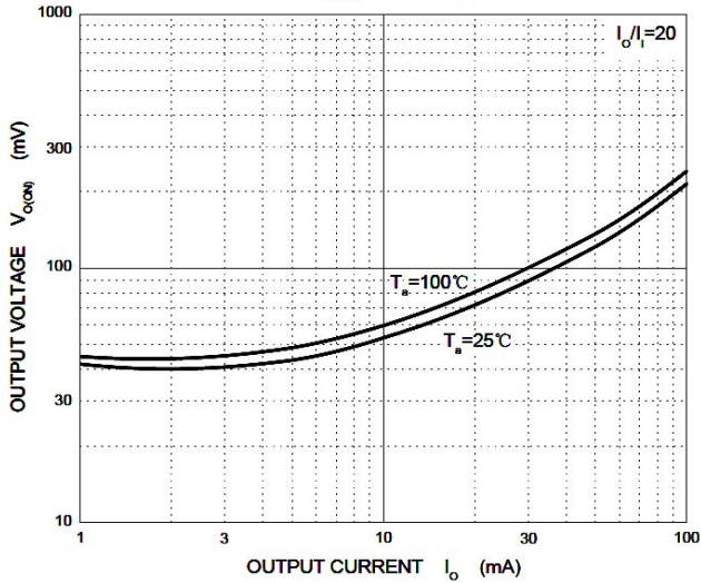
V_{O(ON)} — I_O
