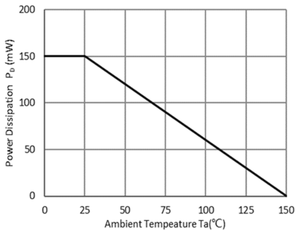
Fig 5: PD-Ta Curve
