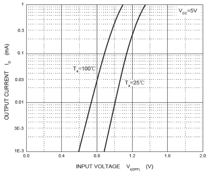
OFF Characteristics
