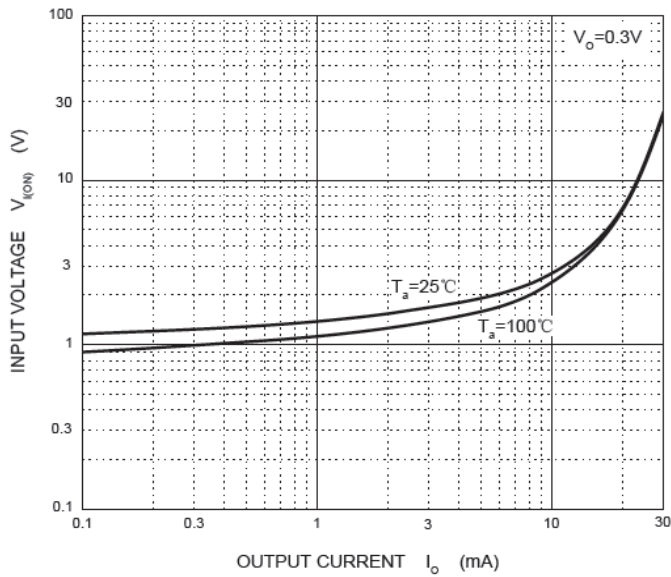
ON Characteristics
