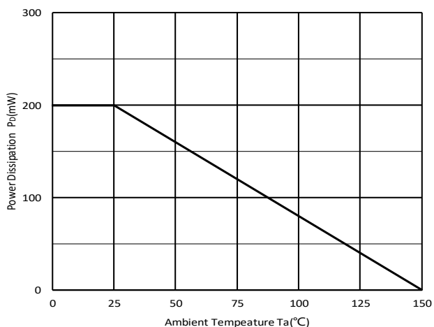
Fig 5: P_D-Ta Curve
