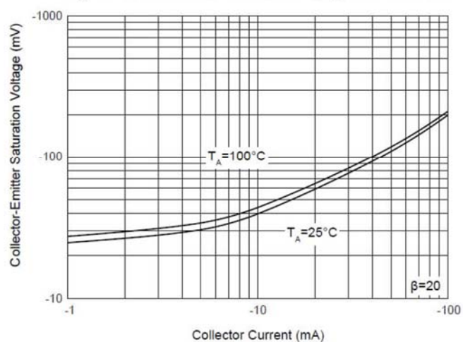
Fig. 2 - Collector-Emitter Saturation Voltage Characteristics
