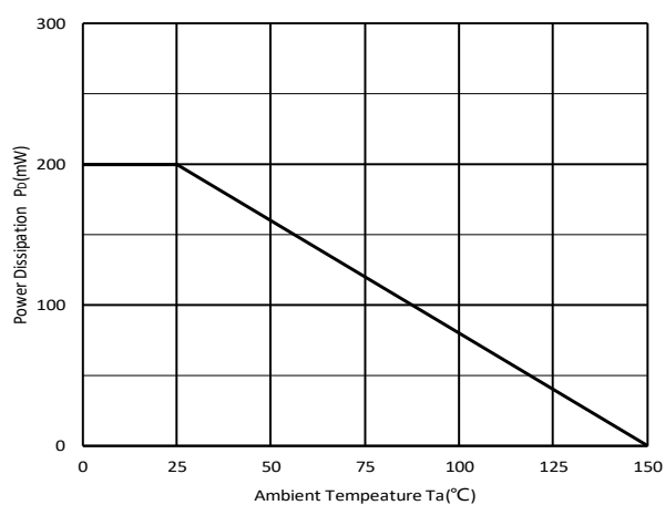
Fig 5: PD-Ta Curve
