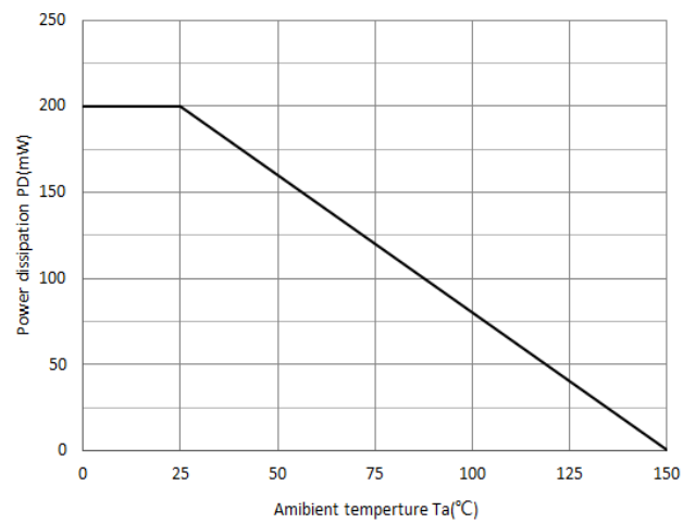
Deratin curve
