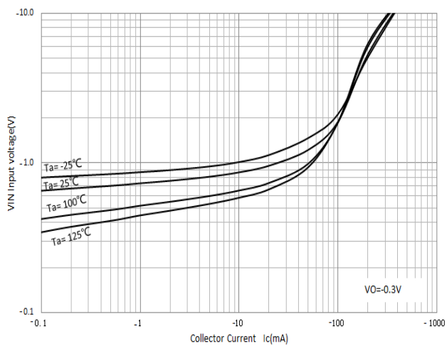
Input voltage vs. collector current
