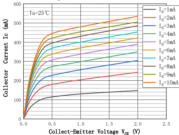
Fig.1-Static Characteristic
